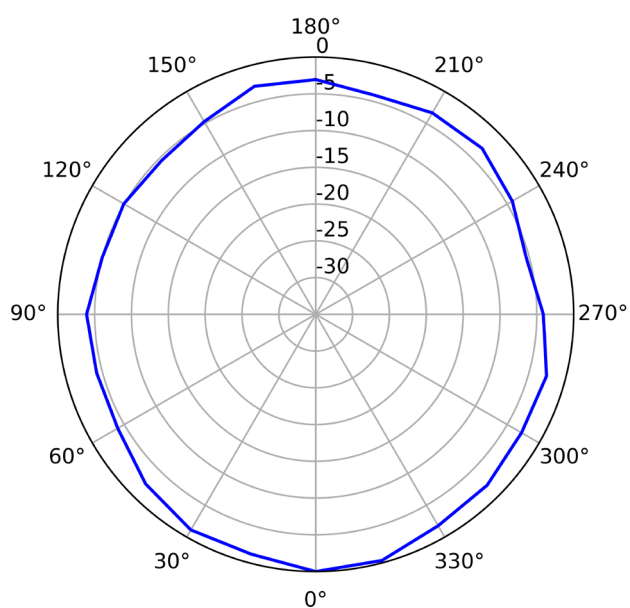
2.4GHz (Horizontal)
