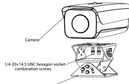
PFA162 3-dimensional universal mounting bracket
